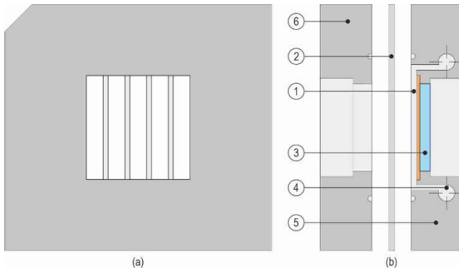
Fig.1. Test module: (a) view from the flow-pattern observation side; (b) longitudinal cross-section: 1 - minichannel, 2 - heated foil, 3 - glass plate, 4 - thermocouple/pressure sensor, 5 - cover (flow-pattern observation side), 6 - cover (IRT measurement side), 7 - copper electrode
