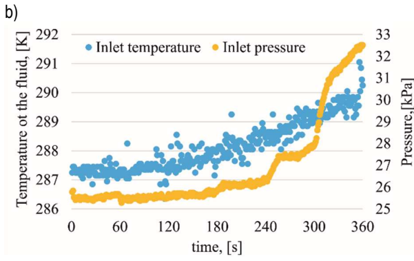
Fig. 2. (a) Temperature of the outer surface of the heating foil, measured by infrared thermography as a function of time and distance from the minichannel inlet, and (b) fluid inlet temperature and pressure as functions of time, for HFE-7100 at a mass flow rate of \dot{m} = 40 kg/h.
